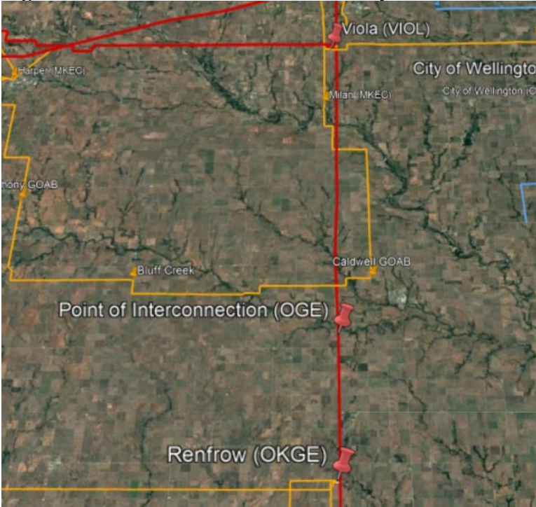
Figure 1 – Renfrow-Viola 345kV line tap
